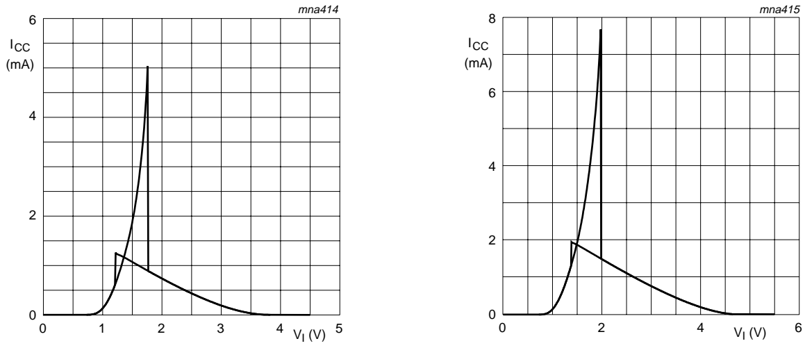
Fig 11. Typical 74VHCT transfer characteristics
